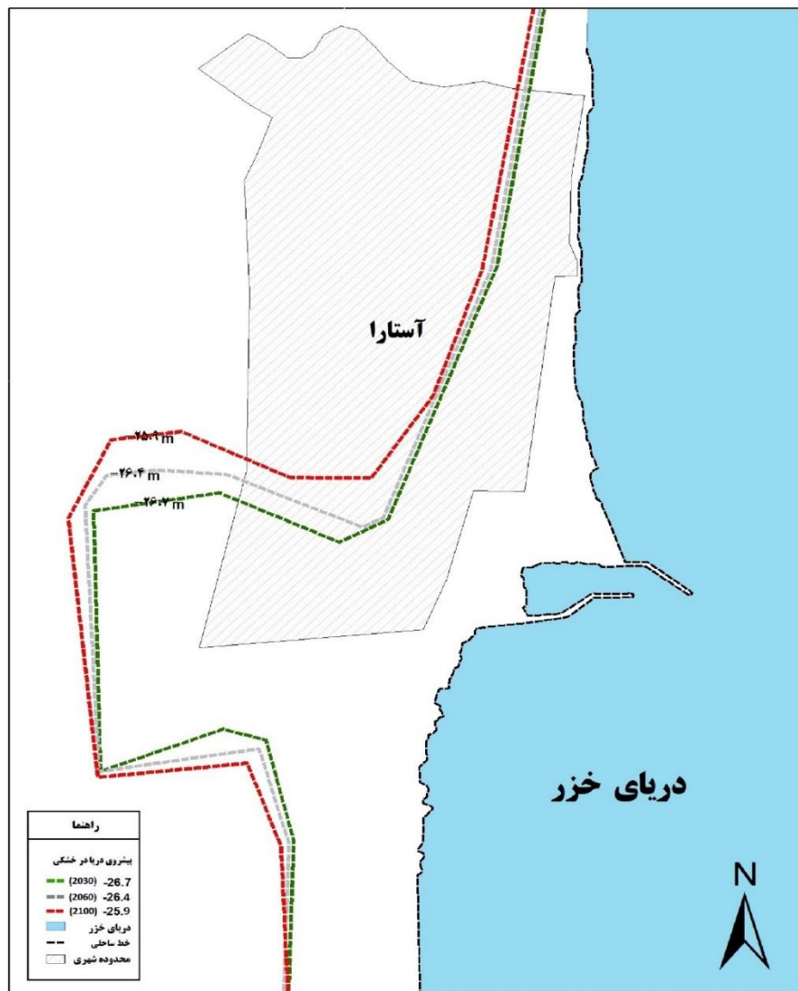
RCP 4.5
